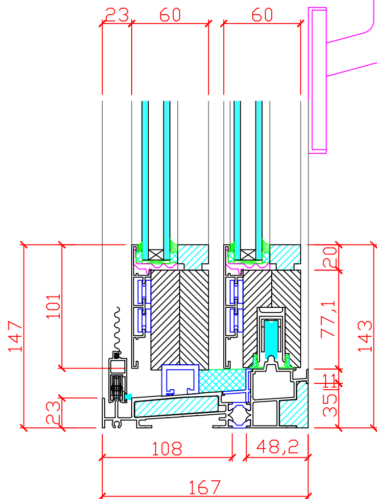
VERTICAL SECTION (A-A')
