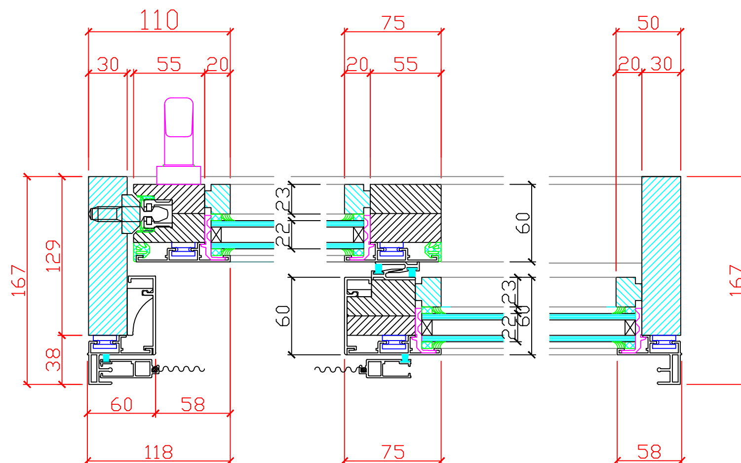
HORIZONTAL SECTION (C-C')
